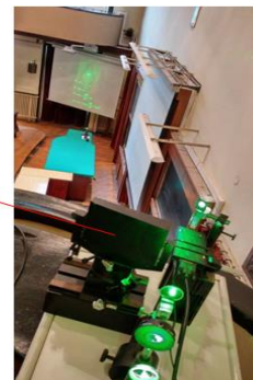
Projection device
